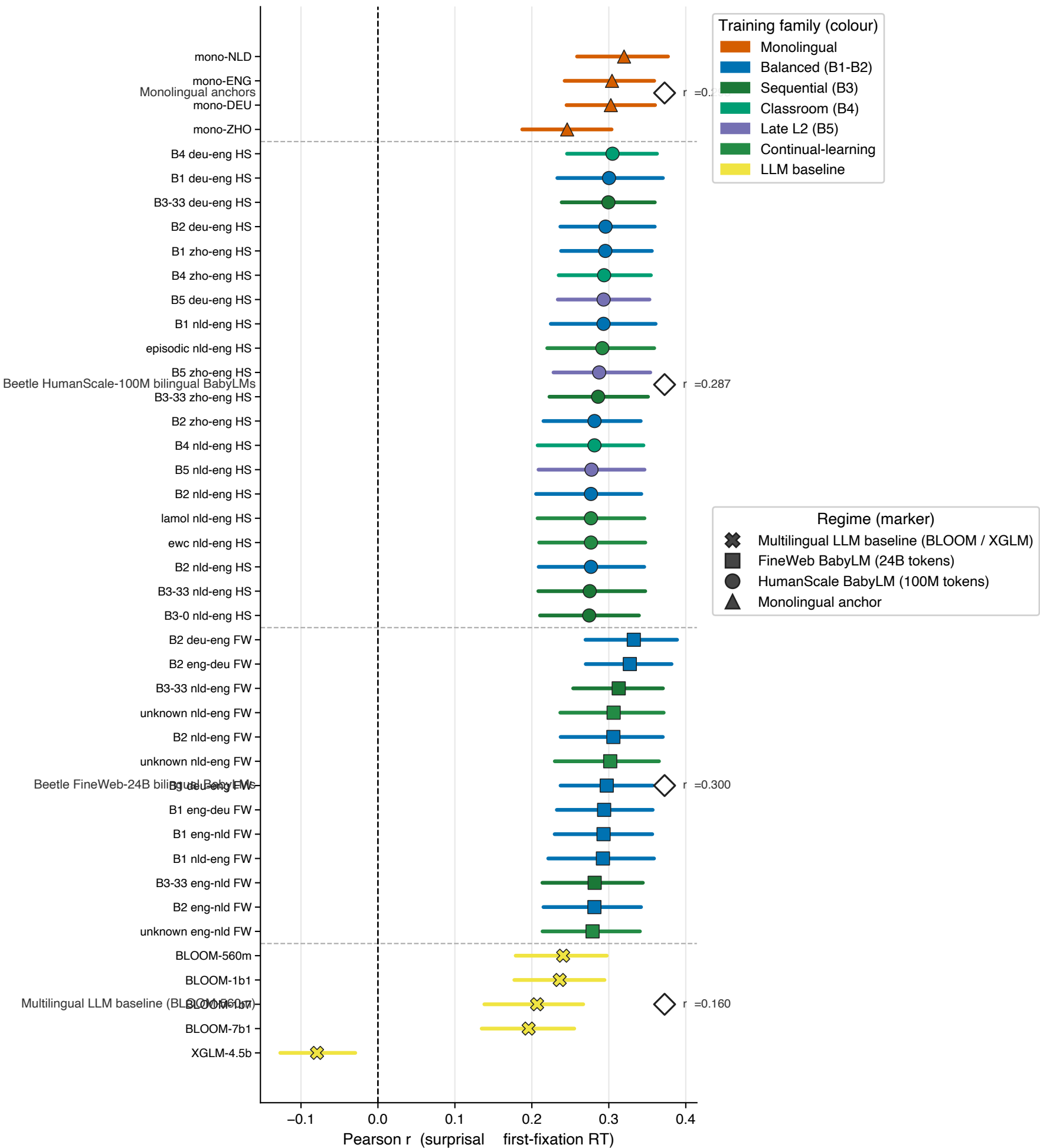
Bilingual BabyLMs match or exceed multilingual LLMs on English L2 cognitive-fit (surprisal RT) MECO L2: English stimuli read by L2-English speakers with diverse L1 backgrounds (Siegelman et al., 2022) Bars = bootstrap 95% CI (n=1000); diamonds on right = group mean r.
